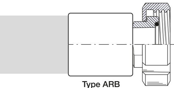
Type ARB (Aseptic Screw Connection, Female) DIN 11864-1 / 11853-1
