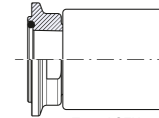
Type ACFN (Aseptic Clamp Flange with Groove, Female) DIN 11864-3 / 11853-3
