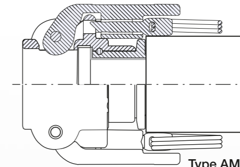
Type ASFN (Aseptic Flange with Groove, Female) DIN 11864-2 / 11853-2
