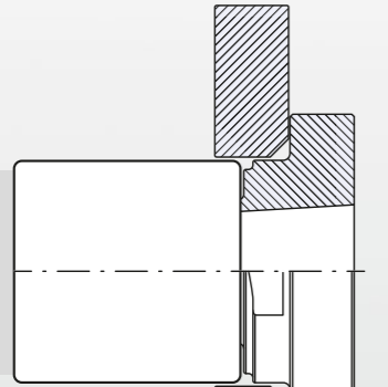
Type SF (Flanged Hose Coupling, Swiveling Flange) EN 1092-1 or ASA (ANSI B 16.5)
