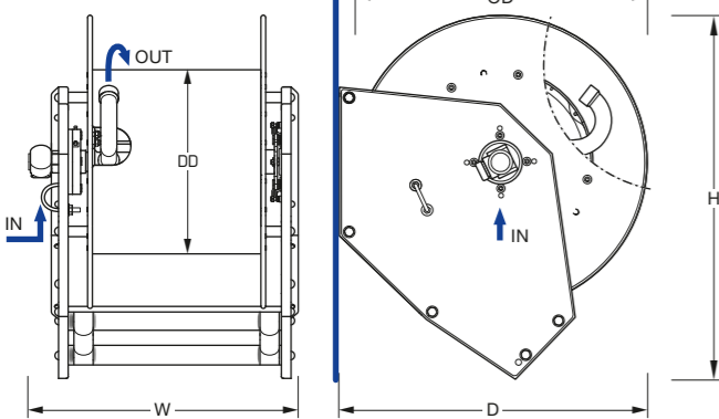
Mounting Position B: Vertical Surface
