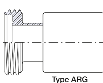
Type ARG (Aseptic Screw Connection, Male) DIN 11864-1 / 11853-1
